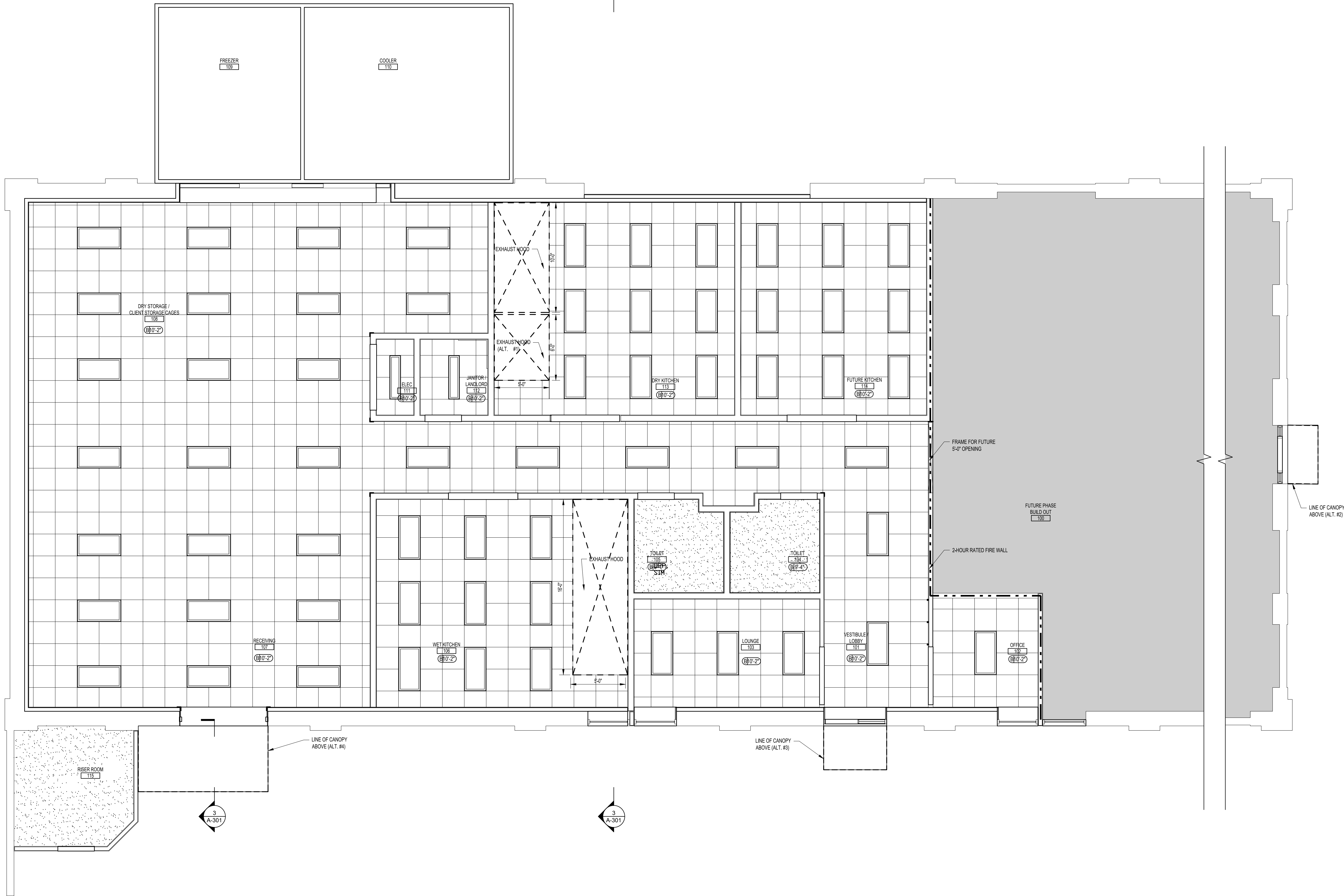
1 REFLECTED CEILING PLAN Scale: 1/4" = 1'-0"
